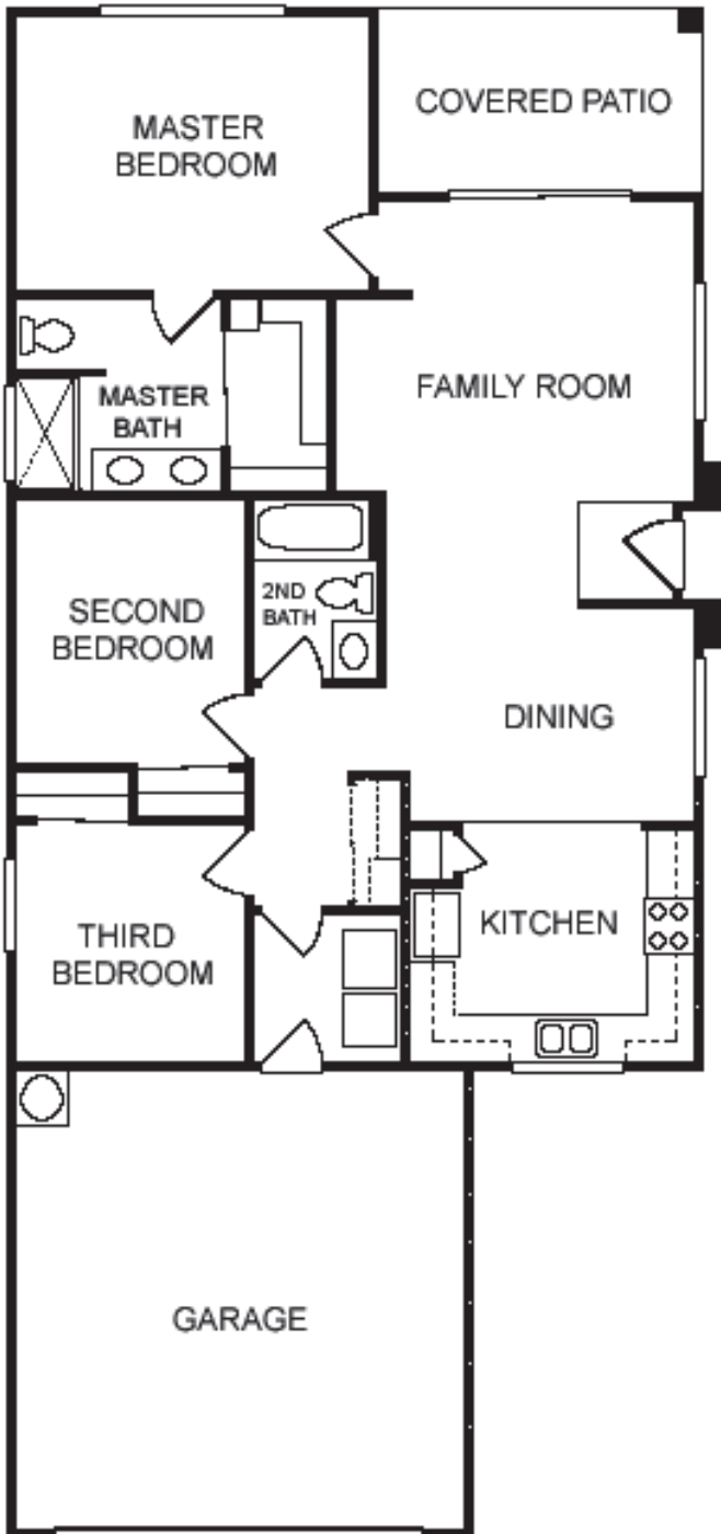
"Palo Verde" Series "Espino" Floorplan
